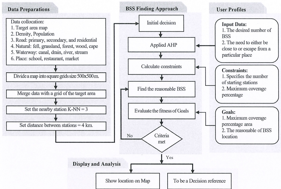
Fig.5: The framework of our proposed methodological.
